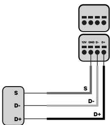
P1 Port
